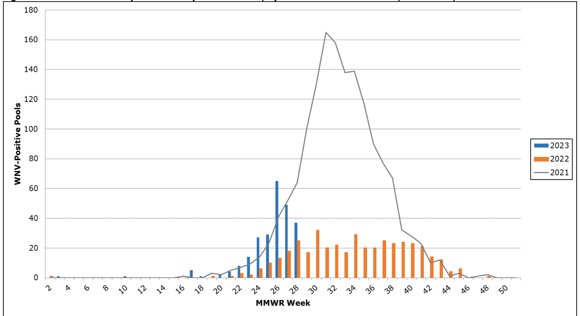
Figure 2. WNV-Positive Mosquito Pools Reported in Texas, by MMWR Week of Collection, 2021-2023, Week 28
