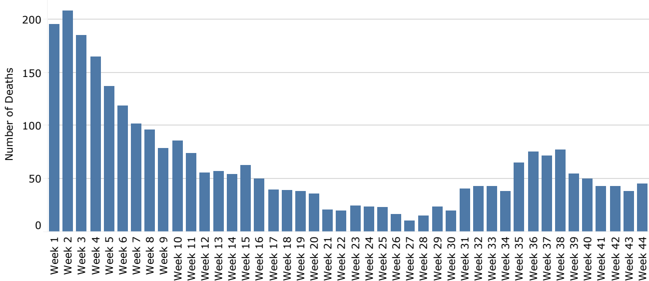
Figure 3: COVID-19 Associated Deaths Identified from Vital Statistics Data by MMWR Week of Death, MMWR Year 2023 Week 44
