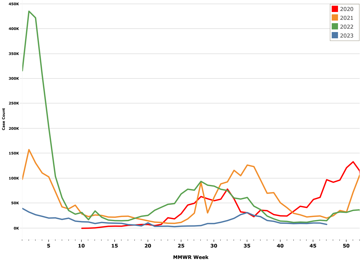
Figure 2: Number of Newly Reported Cases of COVID-19 by MMWR Week, Texas, 2020 to Current Report Week (N = 8,914,358)
